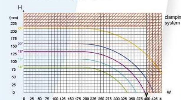
BMT 24NCL Cutting Capacity Chart
