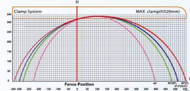
BMT 2036 Cutting Capacity Chart
