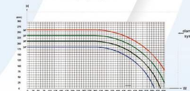
BMT 30NCL Cutting Capacity Chart
