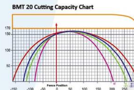
Angular cutting application
