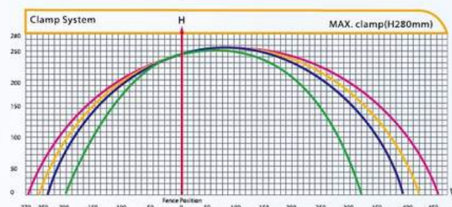
BMT 2030 Cutting Capacity Chart
