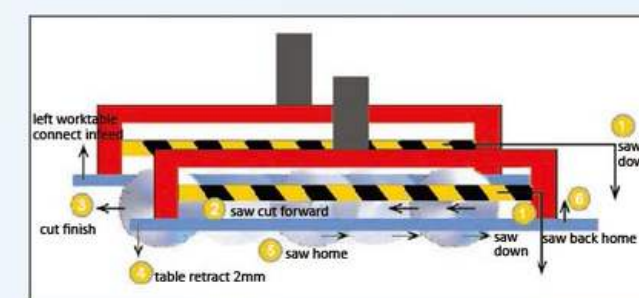
SAWBLADE FEED WAY DIAGRAM
