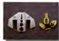
E3 DIE RG TYPE COAXIAL CABLE CONNECTOR 043/068/ 100/137/213/255" 1.09/1.72/2.54/3.48/5.41/6.48 mm RG 58, 59, 62, 174 Fiber Optic
