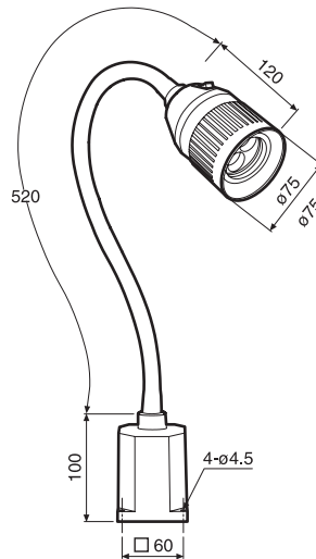
57104535 DIMENSIONS:
