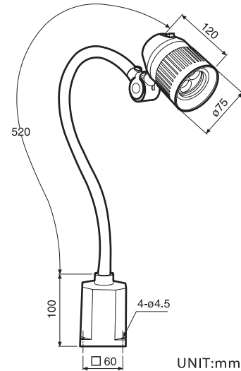
57104536 DIMENSIONS:
