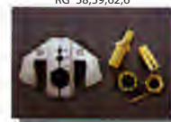
E4 DIE RG TYPE COAXIAL CABLE CONNECTOR 100/ 128/429" 2.54/3.25/10.9 mm RG 8, 11, 174, 179, 213
